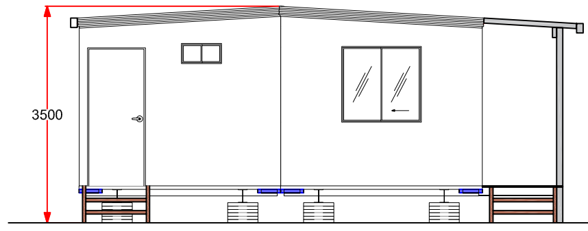
NORTH ELEVATION
