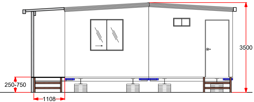
SOUTH ELEVATION
